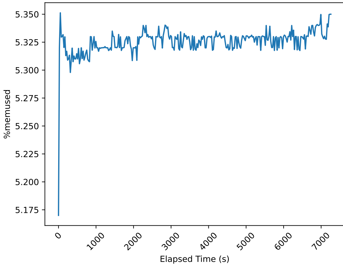
Traces of %memused
